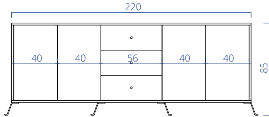
A02CB220 Chi Dolap/ Cabinet
