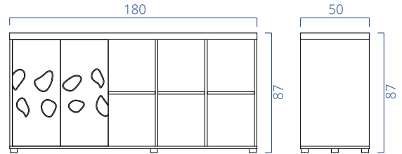
A02DM180 Damla Dolap/Cabinet
